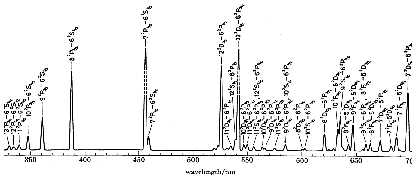
FIGURE 2. Fluorescence-light spectrum obtained in the decay of the selectively excited 12^2D_{3/2} state of Cs, the excitation being 6^1S_0 \rightarrow 6^2P_{3/2} \rightarrow 12^2D_{3/2} . Some of the lines occur because of nearly resonant collision processes (after Belin et al. 1976).
