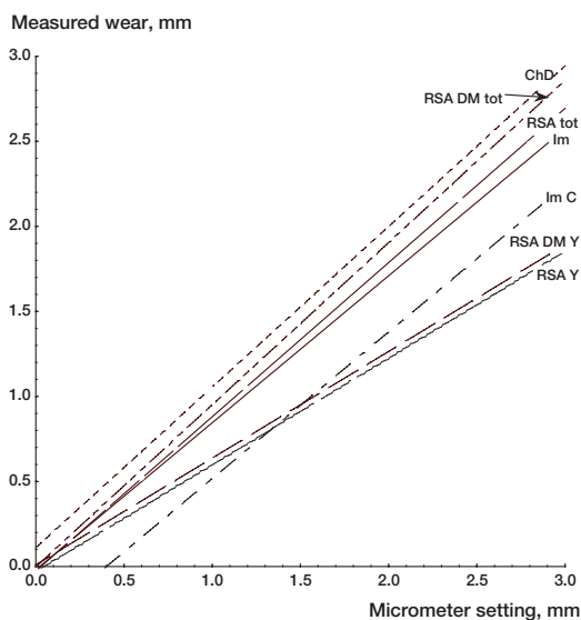
Figure 3. Stage one, regression line with measured wear along the Y-axis and “true” micrometer setting along the X-axis. Im = Imagika, Im C = Imagika™ corrected, ChD = Charnley Duo, RSA Y = RSA along Y-axis, RSA tot = RSA total vector length, RSA DM Y = RSA Digital Measure along Y-axis, RSA DM tot = RSA Digital Measure total vector length.
