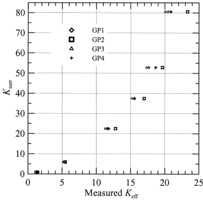
Fig. 2. Measured effective dielectric constant K_{eff} for the four coiled probes before adding gypsum, versus the reference dielectric constants of the surrounding media measured in five different fluids and air.
