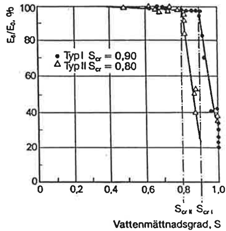
Figure 5: Effect of the degree of saturation on the E-modulus of two types of concrete at a closed freeze-thaw test; /9/.
