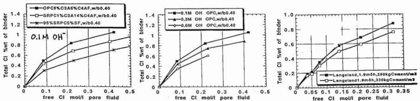
Fig. 1. Examples of chloride binding isotherms. Left : Influence of various binders. Middle : Influence of alkalinity of the pore solution [5,7/]. Right : Field estimations of the relationship total chloride - free chloride for a 15 years old marine upper splash zone concrete, calculated from data presented by Sørensen et al [13/.
