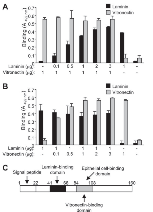
Figure 5. Protein E (PE) is a multifunctional protein that binds both laminin and vitronectin via different regions. A, B , Laminin and vitronectin bind concurrently to PE. A , Increasing laminin concentrations did not influence vitronectin binding to PE. B , Increased concentrations of vitronectin did not influence laminin binding to PE. A, B , PE 22-160 was immobilized and concurrent binding of laminin and vitronectin (micrograms added are shown) were detected by specific antibodies in enzyme-linked immunosorbent assay (ELISA). C , Illustration showing the multifunctional PE. The laminin-binding region is located within PE 41-68 , and the vitronectin and epithelial cell-binding regions are within PE 84-108 [18, 20].
