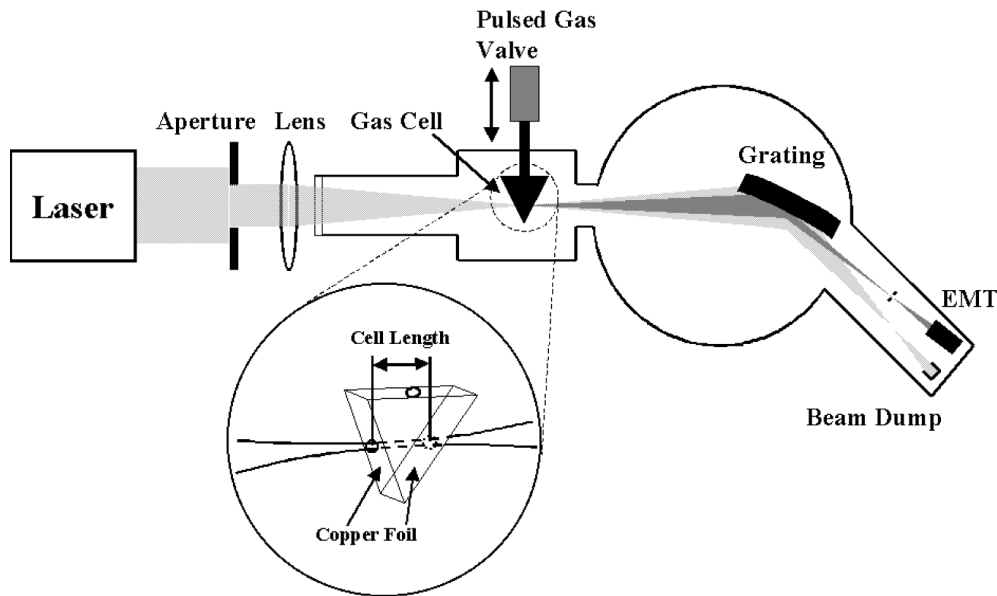
Figure 1. Experimental set-up.
