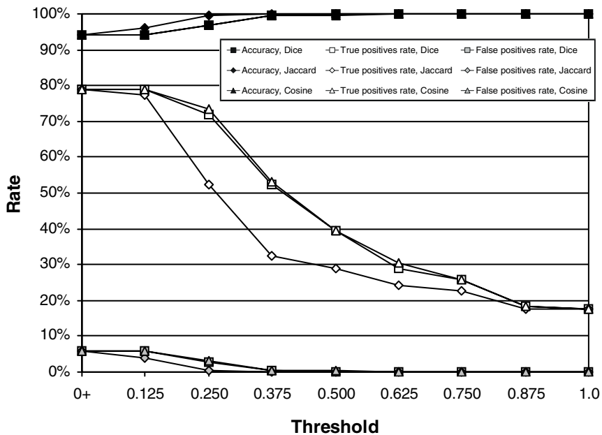
Figure 5b. Similarity analysis performance using the summary field in set B_{reduced} .
