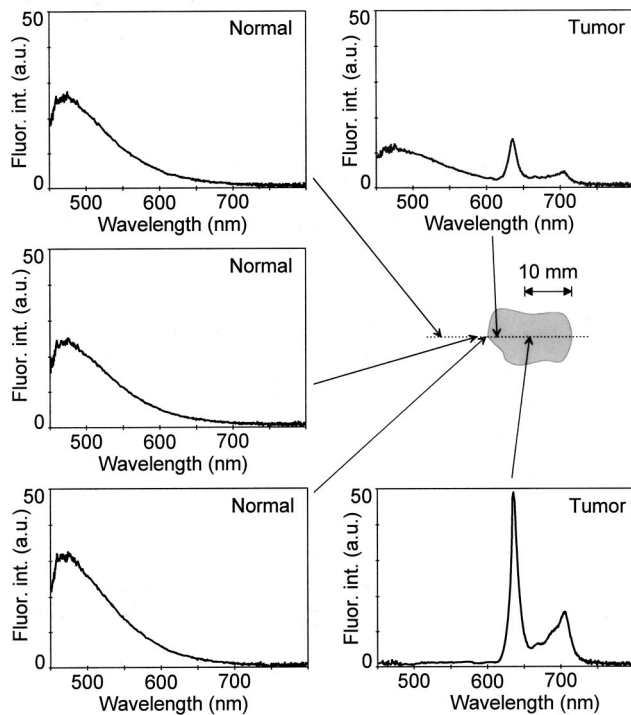
FIG. 3. Fluorescence spectra recorded in a scan across an actinic keratosis, sensitized by a cream containing \delta -amino levulinic acid.
