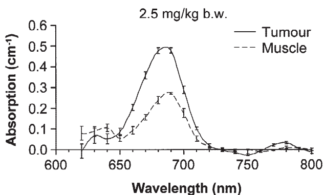
Fig. 6. Plots of the absorption curves for phtalocyanine, recorded for the tumor and for normal surrounding tissue (from af Klinteberg et al. , 1999).
