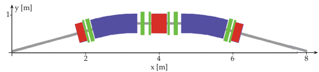
Figure 2: Schematic of one of the twelve DBAs of the MAX IV 1.5 GeV storage ring. Magnets indicated are gradient dipoles (blue), combined quadrupole/sextupole magnets (red), and discrete sextupoles (green).
