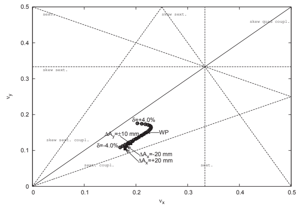
Figure 4: Chromatic and amplitude-dependent tune shifts from the design working point (WP) in fractional tune space. The track point for these studies was at the center of the straight section.
