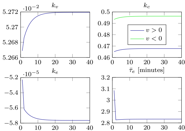
Fig. 8. Estimated parameters from experimental data. The horizontal axis displays the iteration number and the vertical axis displays the current parameter value.
