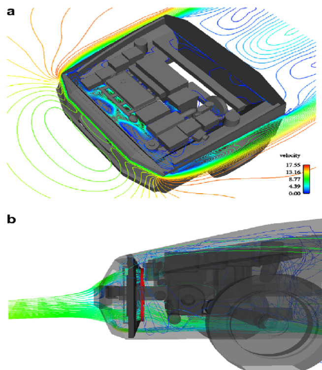
Fig. 11. “a” shows the contours of the air velocity in the vehicle model, “b” shows the air particle traces through a vehicle model [22].
