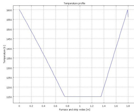
Fig 19. Temperatures profile in furnace and strip
