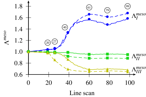
Figure 4: Principal stretches \Lambda_I^{meso} (—●—), \Lambda_{II}^{meso} (---■---) and \Lambda_{III}^{meso} (---▲---) calculated from the DIC fields at two spatial point on the specimen: point A (dashed line) and point B (solid line). The symbols on the curves indicate the line scans for which the stretch fields are presented in Figure 3.
