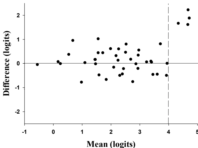
Figure 8 The Bland and Altman graph shows the difference (logits) between the measurements from the two test occasions (test 2 minus test 1) plotted against the mean (logits) of the two test occasions for the ABILHAND (n=43). Four participants (outliers) had high means (>4.0) and large differences in logits between the two test occasions (located to the right of the vertical dashed line).
