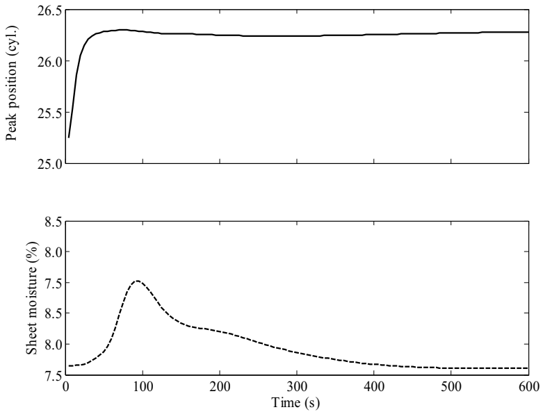
Figure 7.12 Peak position and sheet moisture during the closed loop simulation.
