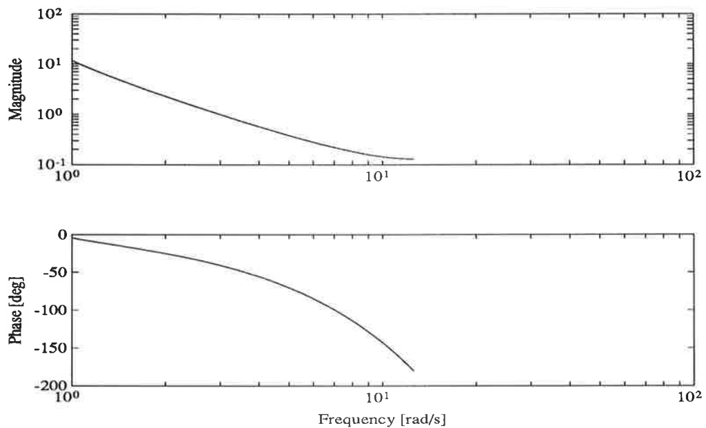
Figure 9: Bode-diagrams of position process, t_{samp} = 0.25s .
