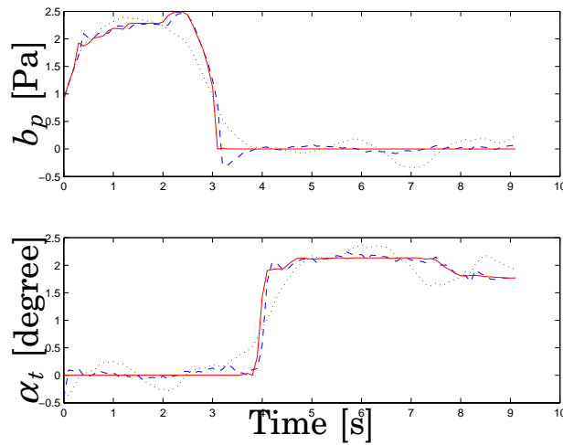
Figure 4.16 Measured b_p and \alpha_t from a driver in a cut-in situation ( solid ). Simulated out data from a 4th order state-space model ( dotted ). Simulated out data from a 4th order one-step ahead predictor ( dashed ).
