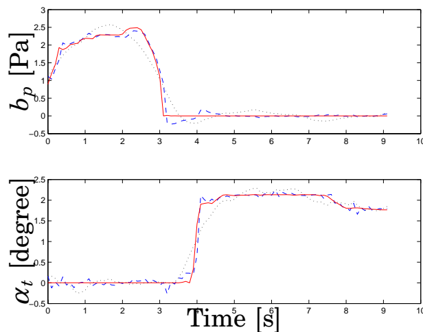
Figure 4.17 Measured b_p and \alpha_t from a driver in a cut-in situation ( solid ). Simulated output data from a 3rd order state-space model ( dotted ). Simulated output data from a 3rd order one-step ahead predictor ( dashed ).
