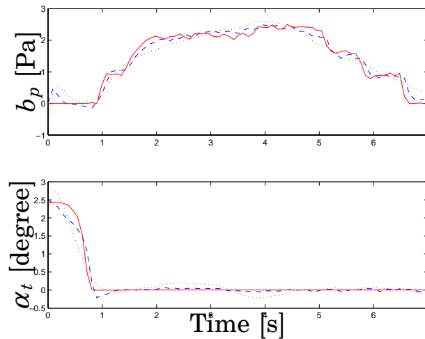
Figure 4.19 Measured b_p and \alpha_t from a driver in a braking situation ( solid ). Simulated out data from a 3rd order state-space model ( dotted ). Simulated output data from a 3rd order one-step ahead predictor ( dashed )
