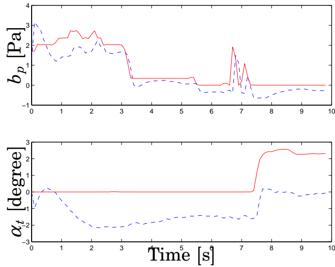
Figure 4.18 Cross validation: measured b_p and \alpha_t from a driver in a cut-in situation ( solid ) not used in the model estimation. Simulated output data from a 4th order one-step ahead predictor ( dashed ).
