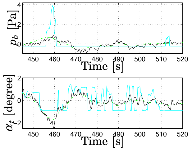
Figure 4.10 Measured b_p and \alpha_t from one driver ( grey ) and simulated output data from state-space models using subspace-based methods, n = 5 ( dashdot ), and n = 15 ( solid ). Normalized and detrended brake pressure and throttle angle was used.
