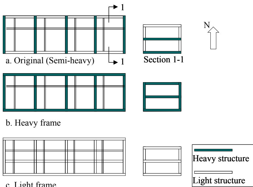
Figure 6.2 General layout of three different frames
