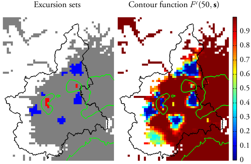
Figure 9: Results from the \text{PM}_{10} application for January 30, 2006. In the left panel, the set E_{50,0.1}^+(x) is shown in red, E_{50,0.1}^-(x) in blue, and its complement E_{50,0.1}^+(x)^c in grey. The contour curve for the level 50\mu\text{g}/\text{m}^3 is shown in green. The right panel shows the contour function for the level 50\mu\text{g}/\text{m}^3 , F^c(50, s) .
