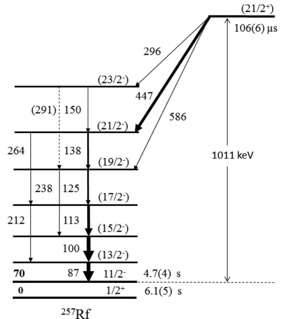
FIG. 4. Decay scheme of the high- K isomeric state in ^{257}\text{Rf} . The energies are in kilo electron volts and the arrow widths correspond approximately to the transition intensities. The energy of the 11/2^{-} state could not be determined in this work and has been taken from Ref. [21].
