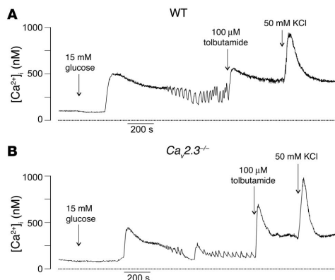
Figure 3 Ca^{2+} homeostasis in WT and Ca_v2.3^{-/-} islets. (A) [Ca^{2+}]_i in an intact WT Ca_v2.3^{+/+} islet assayed by ratiometric fura-2 measurements. The islets were stimulated at the time points indicated by the arrows in the continued presence of previously added stimuli. (B) [Ca^{2+}]_i was determined as in A, but the experiment was performed in an intact Ca_v2.3^{-/-} islet. Recordings selected for display are representative of 7 and 9 separate experiments in WT and Ca_v2.3^{-/-} islets, respectively. Statistical significances are provided in the text.
