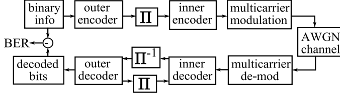
Figure 2.11: System setup of FTD transceiver to evaluate the decoder performance.
