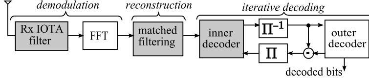
Figure 5.1: Block diagram of the FTN receiver chain.
