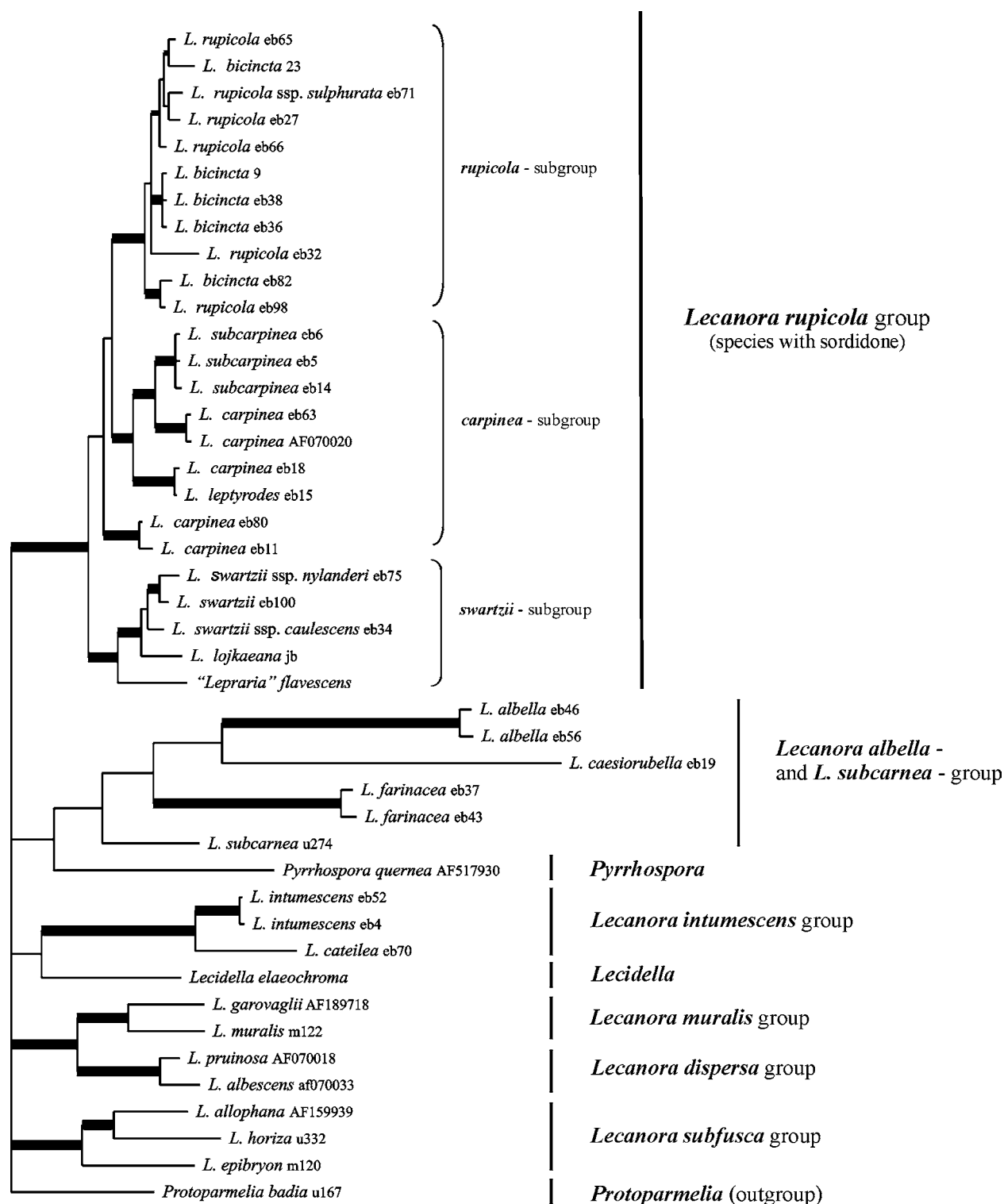
Fig. 2. 50% Majority-rule consensus tree based on 19 001 trees from a B/MCMC tree sampling procedure. Posterior probability supports are indicated in thickness of the internodes: — <90%, — 90–94%, — 95–100%.
