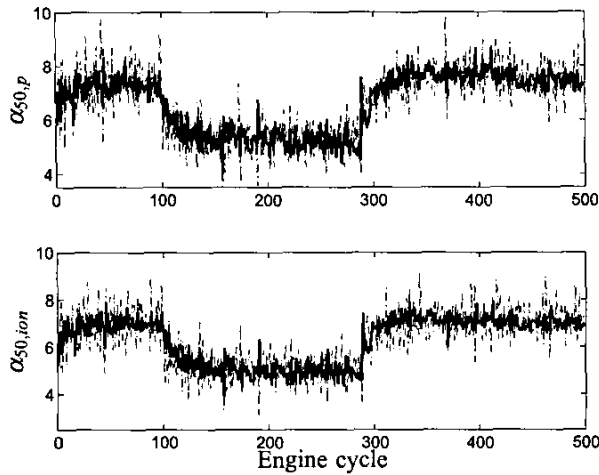
Fig. 14. Responce in \alpha_{50,p} and \alpha_{50,ion} to step changes in CA50 reference. Upper figure: 3-step ahead predicted model output (black) and \alpha_{50,p} (grey). Lower figure: 3-step ahead predicted model output (black) and \alpha_{50,ion} (grey)
