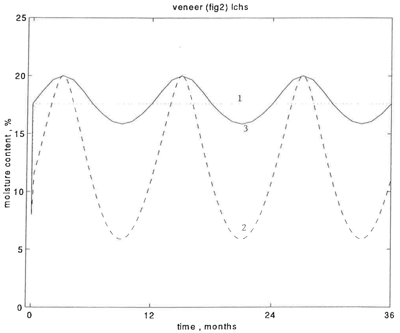
Figure 4. Simulation for the 1 mm veneer (A).
