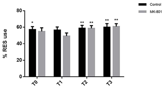
Figure 3 | The effects of NMDA receptor antagonist MK-801 (0.1 \mu\text{M} ) treatment on long term memory retrieval in 10 dpf zebrafish. Individuals were familiarized with novel objects for 2 hours in a massed paradigm. Individuals were moved to a fresh media without treatment for 23 hours, after which MK-801 was administered. Reintroduction of the objects occurred 1 hour after MK-801 administration. Controls have a significant RES preference at T0 ( t = 2.00 , p = 0.051 ), T2 ( t = 3.44 , p = 0.022 ) and T3 ( t = 4.26 , p = 0.023 ). MK-801-treated individuals displayed RES preference at T2 ( t = 3.23 , p = 0.012 ) and T3 ( t = 3.47 , p = 0.003 ). Significance * p < 0.05 , ** p < 0.001 , *** p < 0.0001 , computed using single sample t-test tested against 50%. For control and MK-801 treated groups, n = 36 . Error bars indicate SEM.
