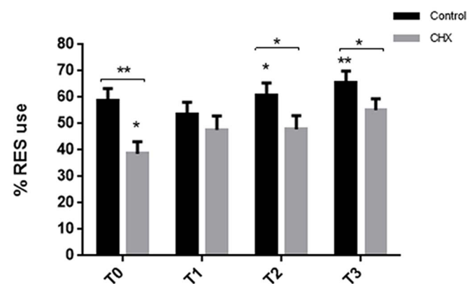
Figure 4 | 10 dpf zebrafish larvae demonstrate protein synthesis-dependent long-term NOR. Controls and CHX treated (10 \mu\text{M} ) individuals were familiarized with novel objects for 2 hours in a massed paradigm. Individuals were moved to a fresh media without treatment for 24 hours and then reintroduced with the objects. CHX-treated individuals show RES preference at T0 ( t = -2.49 , p = 0.018 ). Controls had RES preferences at T2 ( t = 2.46 , p = 0.019 ) and T3 ( t = 3.74 , p < 0.001 ). Significance * p < 0.05 , ** p < 0.001 , *** p < 0.0001 , computed using a single sample t-test tested against 50%. For control and CHX treated groups, n = 36 . Error bars indicate SEM.
