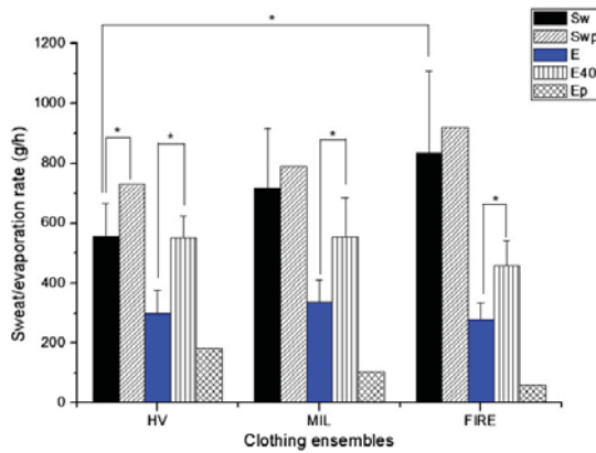
Figure 3. The mean sweat rate Sw , the predicted sweat rate Swp , the mean evaporation rate E , the predicted evaporation rate Ep and the evaporation rate E40 calculated from the last 40 min exposure during HV, MIL and FIRE at 40.0 °C. * p < 0.05 .
