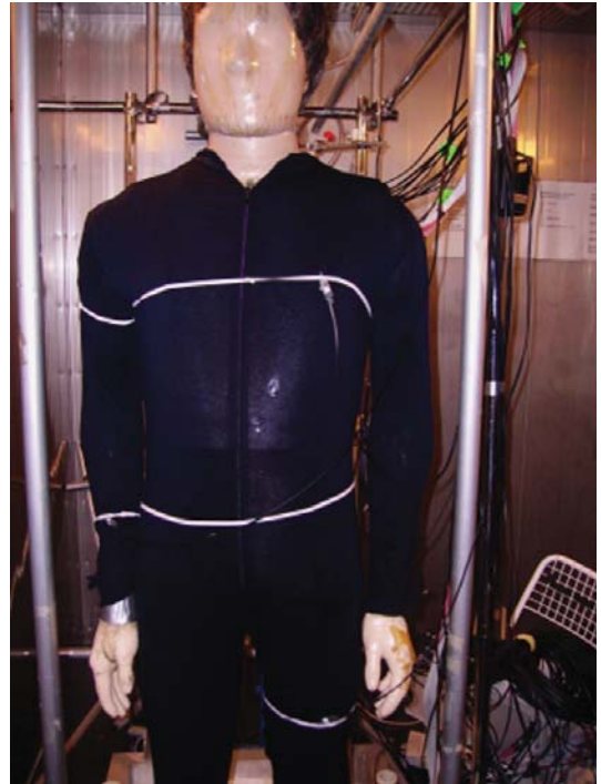
Fig. 1. The thermal manikin 'Tore' in the climatic chamber.
