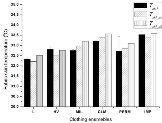
Fig.4.2 Observed and predicted fabric skin temperatures for 6 clothing ensembles. T_{sk,f} , the observed fabric skin temperature; T_{skf\_p1} , the predicted fabric skin temperature by Eq.(4-1); T_{skf\_p2} , the predicted fabric skin temperature by Eq.(4-2). [Reprinted with permission]
