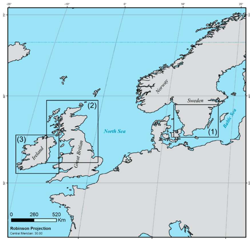
Fig. 6. Location of study areas in the context of north-west Europe. (1) Southern Swedish study area. (2) British study area. (3) Irish study area. Base mapping is ©ESRI, modified and re-drawn from ESRI ArcGIS template 'Europe'.
