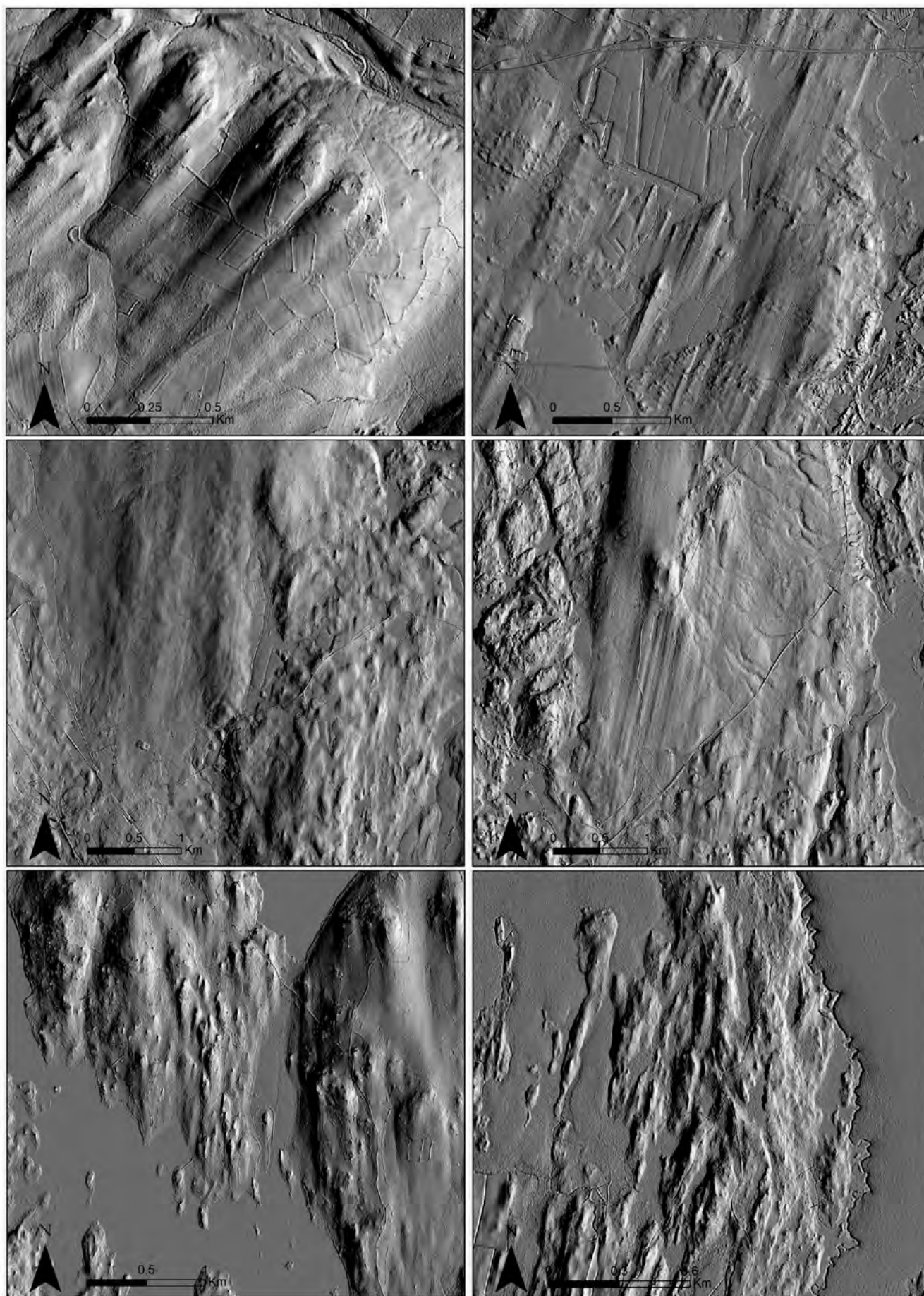
Fig. 2 Examples of drumlinoids in their natural habitat. Images are generated from the 2 m resolution Swedish national height model—the height data is hill-shaded with illumination azimuth at 90°, altitude at 25° and a x5 vertical exaggeration. These images are taken from southern Swedish region and illustrate the range in shape and size found.
