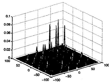
Fig. 7 The amplitude plot of the HTF H_{loco} . Notice the large out-diagonal bands, illustrating the nonlinear coupling between different frequencies in V_{line} and I_{AC} .
