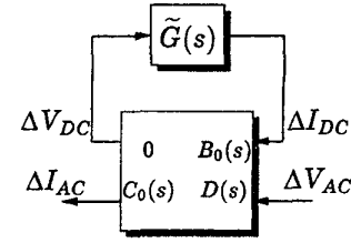
Fig. 5 The diode converter with the DC dynamics \tilde{G}(s) connected. The resulting HTF, H_{db}(s) , is then connected with a model of the transformer \tilde{Z}_{traf}(s) , see Fig. 6.
