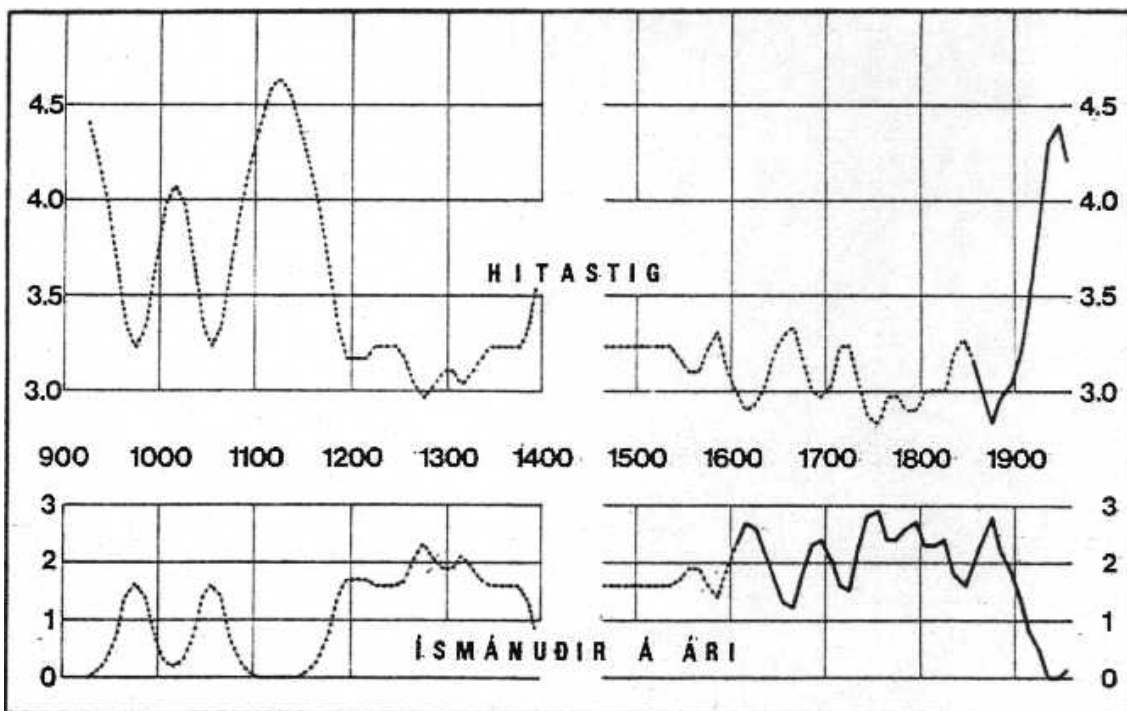
Fig 5.2.2. Running 30-year means of temperature (top) and ice incidence in months per year (below). Estimated values: dotted line (from Bergþórsson 1969).
