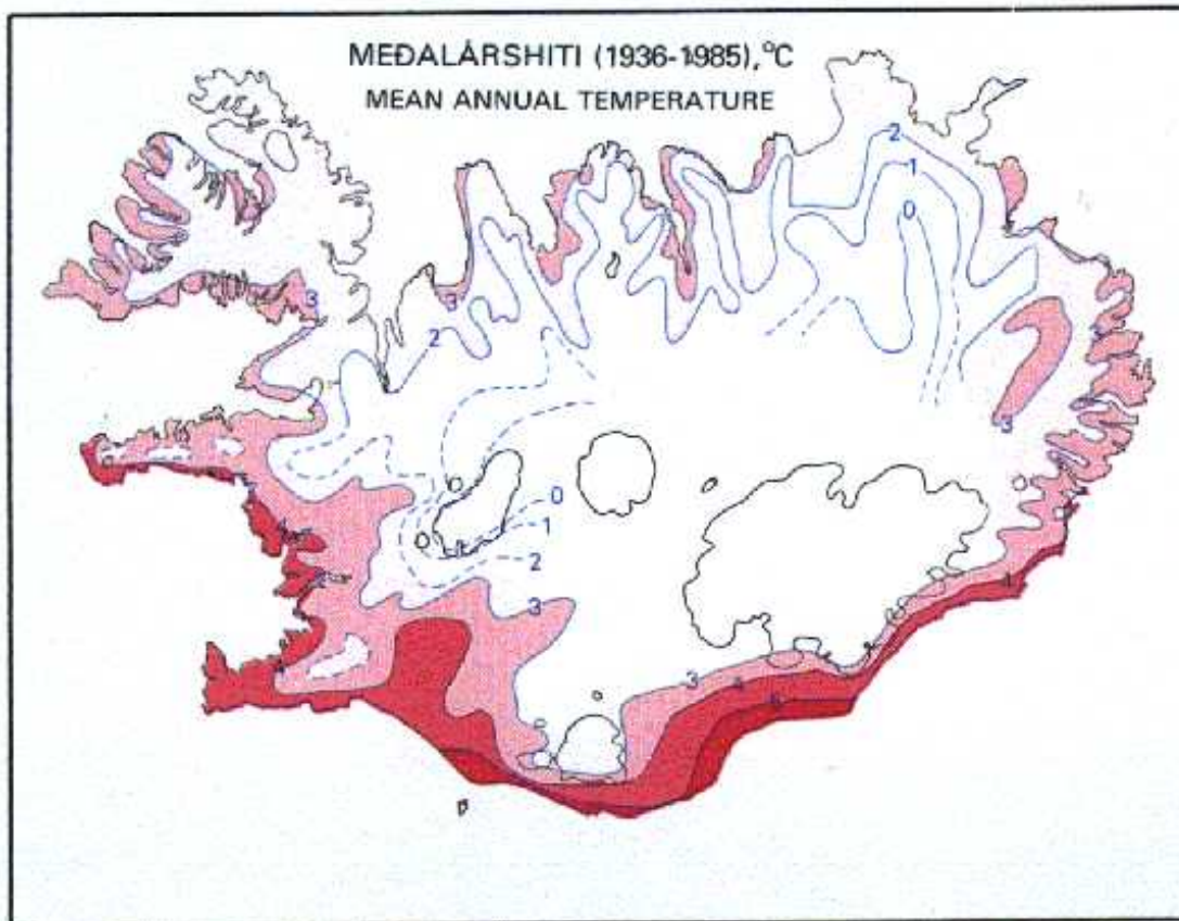
Fig. 3.2.1a. Mean annual temperature 1936-1985 (°C) (from IGI/LMÍ 1996)
