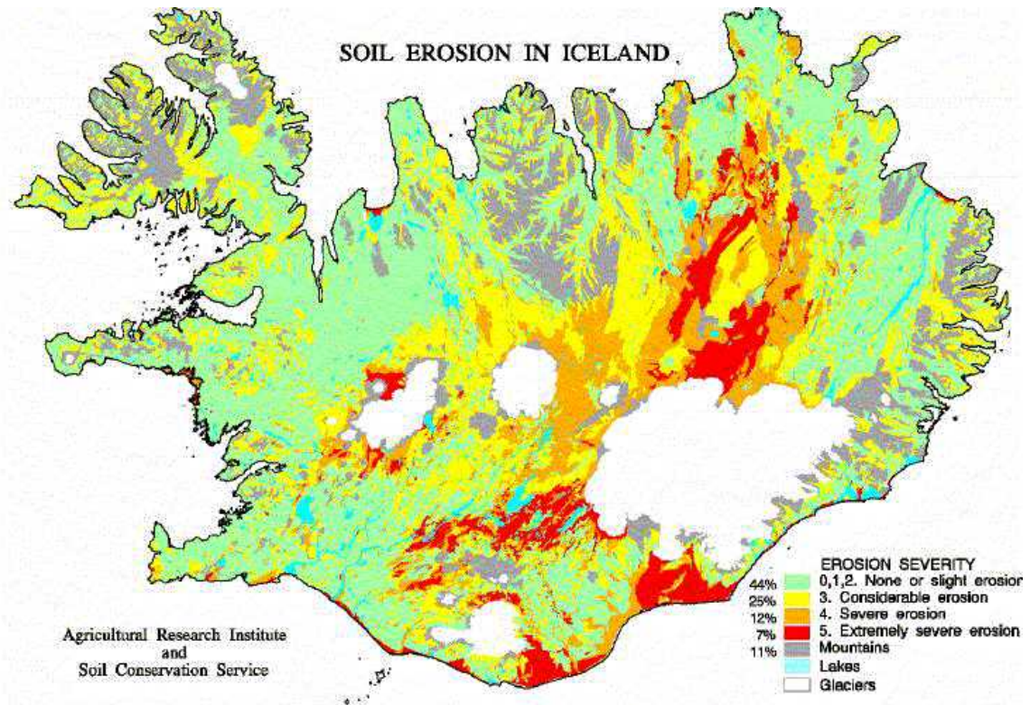
Fig 3.6.3. Erosion map from Arnalds et. al. 1997. For further information please refer to http://www.rala.is/desert .
