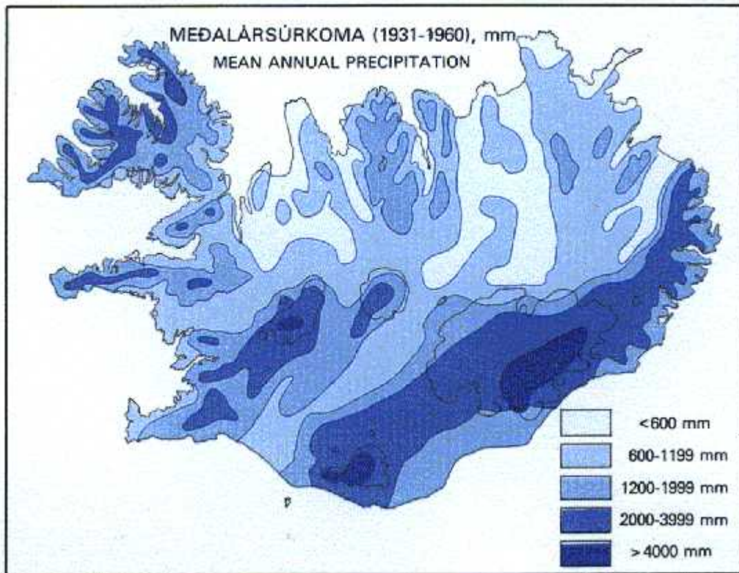
Fig. 3.2.1b Mean annual precipitation 1931-1960 (mm) (IGI/LMÍ 1996)
