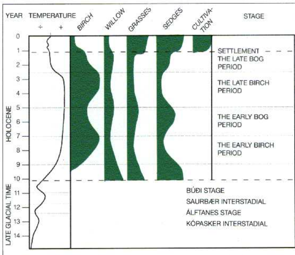
Fig. 3.4.1. Changes in mean annual temperature and vegetation from late glacial time and the Holocene in Iceland. Furthest to the left thousands of years BP. The curves show proportional changes in vegetation and apply mainly to the south of the country. (From Einarsson P. 1994)
