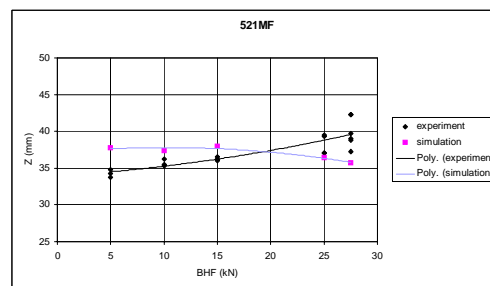
Figure 7. Springback as function of the blank holder force. The diagrams show the results for the aluminium (521MF).
