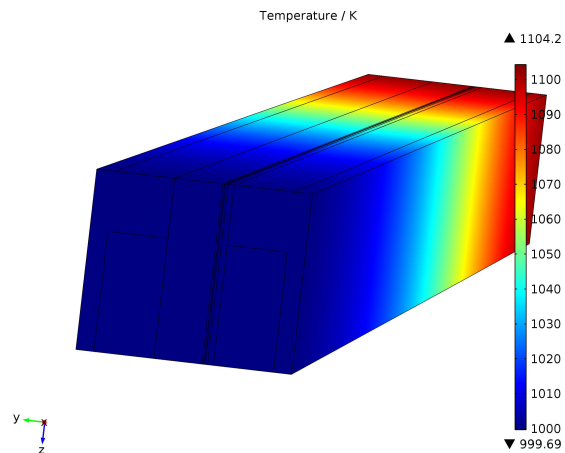
Figure 2. Temperature distribution in 3D for the standard case.
