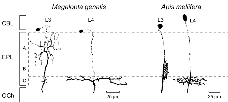
Figure 6. Comparison of the First-Order Interneurons, L-fiber types L3 and L4, of the M. genalis female ( left ) and the worker honeybee A. mellifera ( right )
