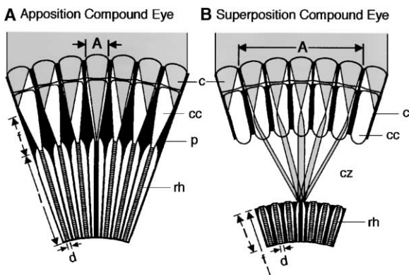
Figure 1. Schematic Diagrams of the Two Main Compound-Eye Designs
