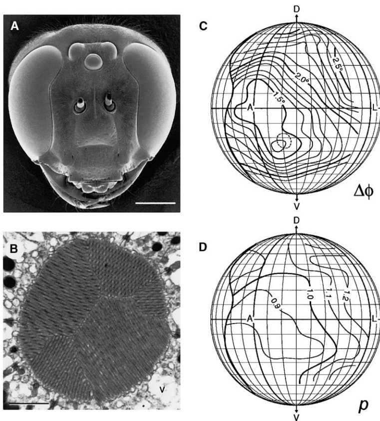
Figure 3. The Apposition Eyes of Megalopta (A) A scanning electron micrograph of the head of a female Megalopta genalis (antennae removed for clarity). Note the three very large ocelli. Large ocelli are typical of nocturnal bees and wasps [12, 14, 72]. The scale bar represents 1 mm.
