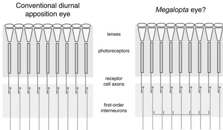
Figure 5. A Possible Mechanism for Spatial Summation in Megalopta's Eye
