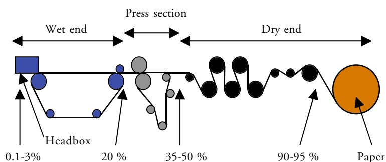
Figure 2.3 Schematic outline of a paper machine. The numbers are approximate values of the dry substance in the transformation of stock into paper.
