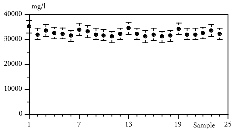
Figure 2.7 Concentration of dissolved COD (•) in whitewater from mill no. 2 during sampling period 010924.
