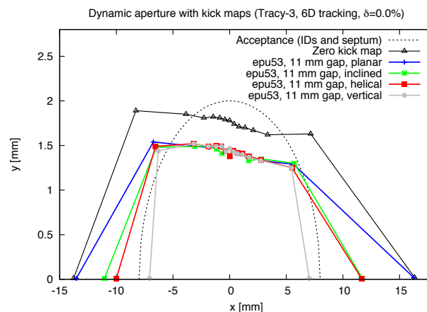
Figure 3: Tracking of DA of the MAX IV 3 GeV storage ring with Tracy-3 using kick maps to show the effect of epu53 in different modes.
