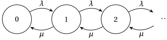
Figure 2.2 State diagram of an M/M/1 queueing system with arrival rate \lambda and service rate \mu .
