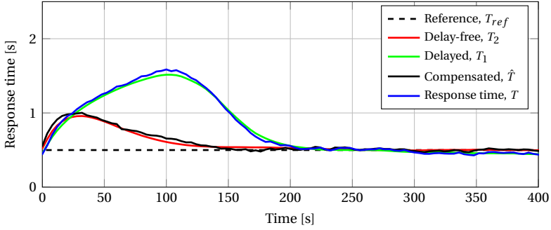
Figure 4. Response time results from simulation of step up. The compensated response times reach the reference much before the actual response times.
