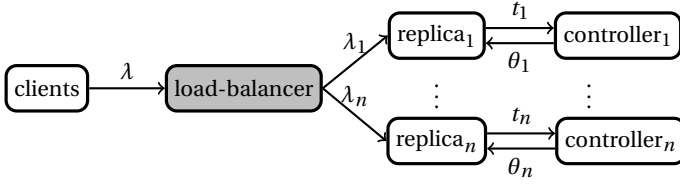
Figure 2.1 System architecture of replicated brownout applications as in Papers I and II. User requests to the application are dispatched to indepent replicas of the application by a load balancer. Each replica contains a separate brownout controller that maintains the response time of its respective replica.
