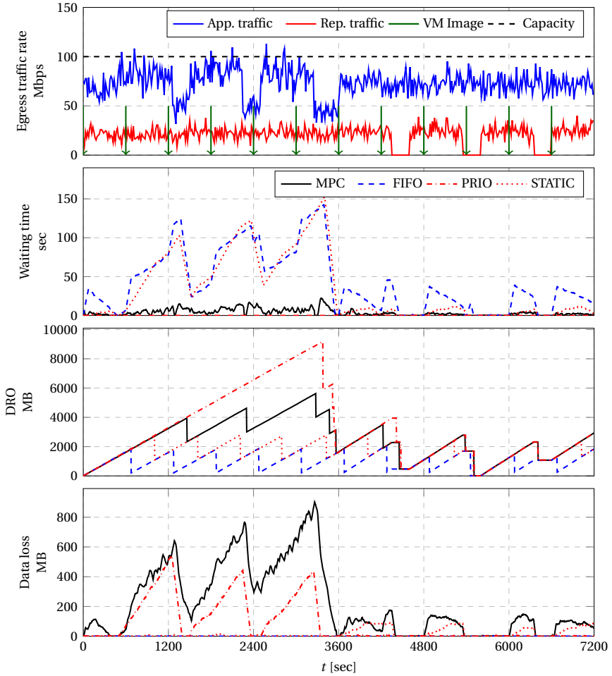
Figure 4. Results from experiment 2. Figures as in Figure 3.
