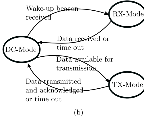
Figure 1: (a) Simplified node architecture block diagram, with signaling in listen/receive mode shown. (b) State-transition diagram of overall operation of a node for the DCW-MAC scheme.
