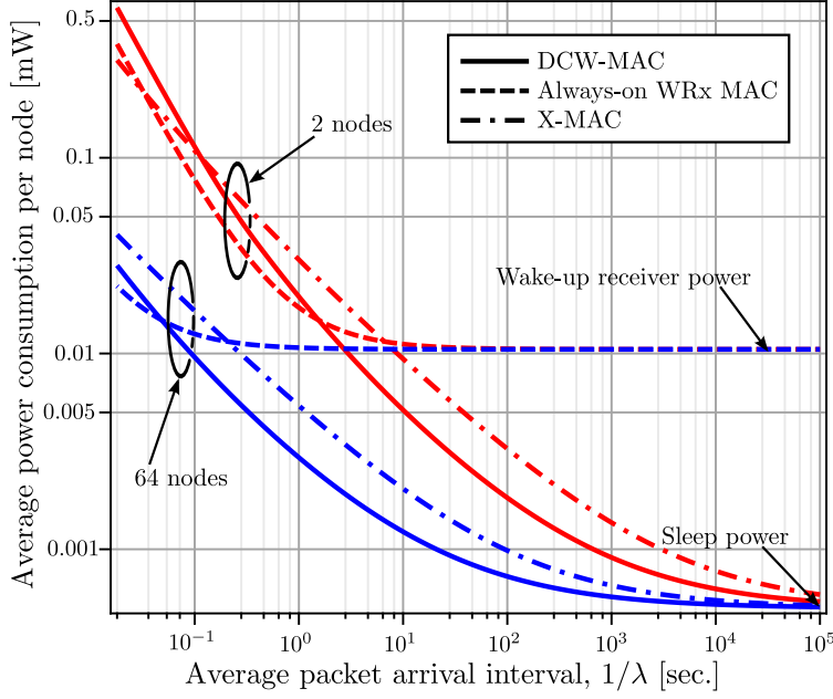
Figure 8: Average power consumption per node vs. average packet arrival interval.
