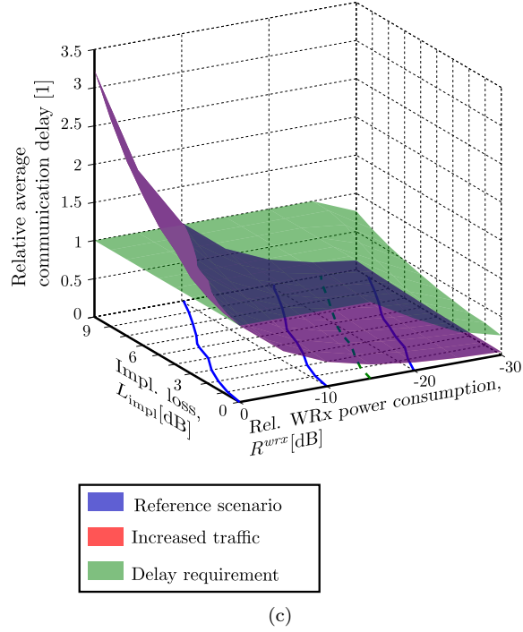
Figure 5.6: 3D illustration of DCW-MAC (a) energy savings relative to X-MAC, (b) energy savings relative to Always-On WRx-MAC, and (c) average communication delay, together with their corresponding level curves, for three different scenarios. The reference scenario has a 1000 sec. 1/\lambda and no delay requirement. Based on the reference scenario, the other two scenarios have traffic increased to a 10 sec. 1/\lambda and a 0.1% relative delay requirement, respectively. Results are shown for an 8-bit address space.
