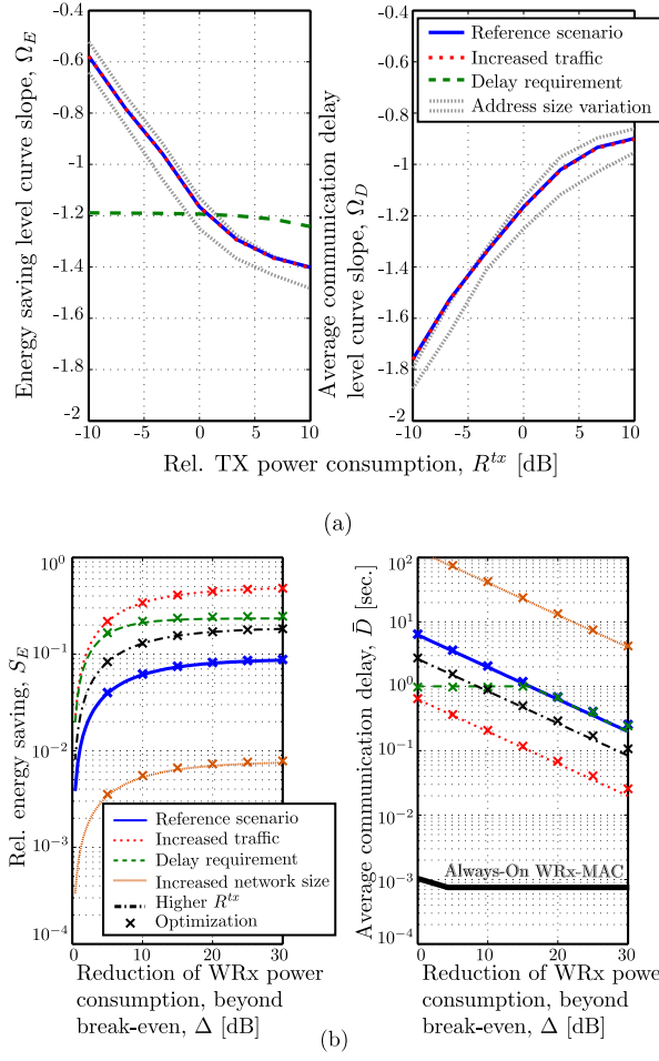
Figure 7: (a) Level curve slopes \Omega_E and \Omega_D for different relative transmit power consumptions. (b) Comparison of optimal values (crosses) and corresponding approximations (lines) of energy savings and average communication delays, for different WRx power reductions beyond break-even ( \Delta ) without implementation loss.
