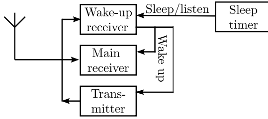
Figure 1: Simplified node block diagram. The transmitter is used both for data and wake-up beacon (WB) transmission, while the main receiver and wake-up receiver (WRx) are used for data and WB reception, respectively. The sleep timer is used when we have duty-cycled WRx scheme.
