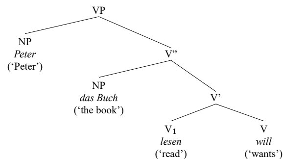
Figure 13.1: The structure of the VP Peter das Buch lesen will ('Peter wants to read the book')
