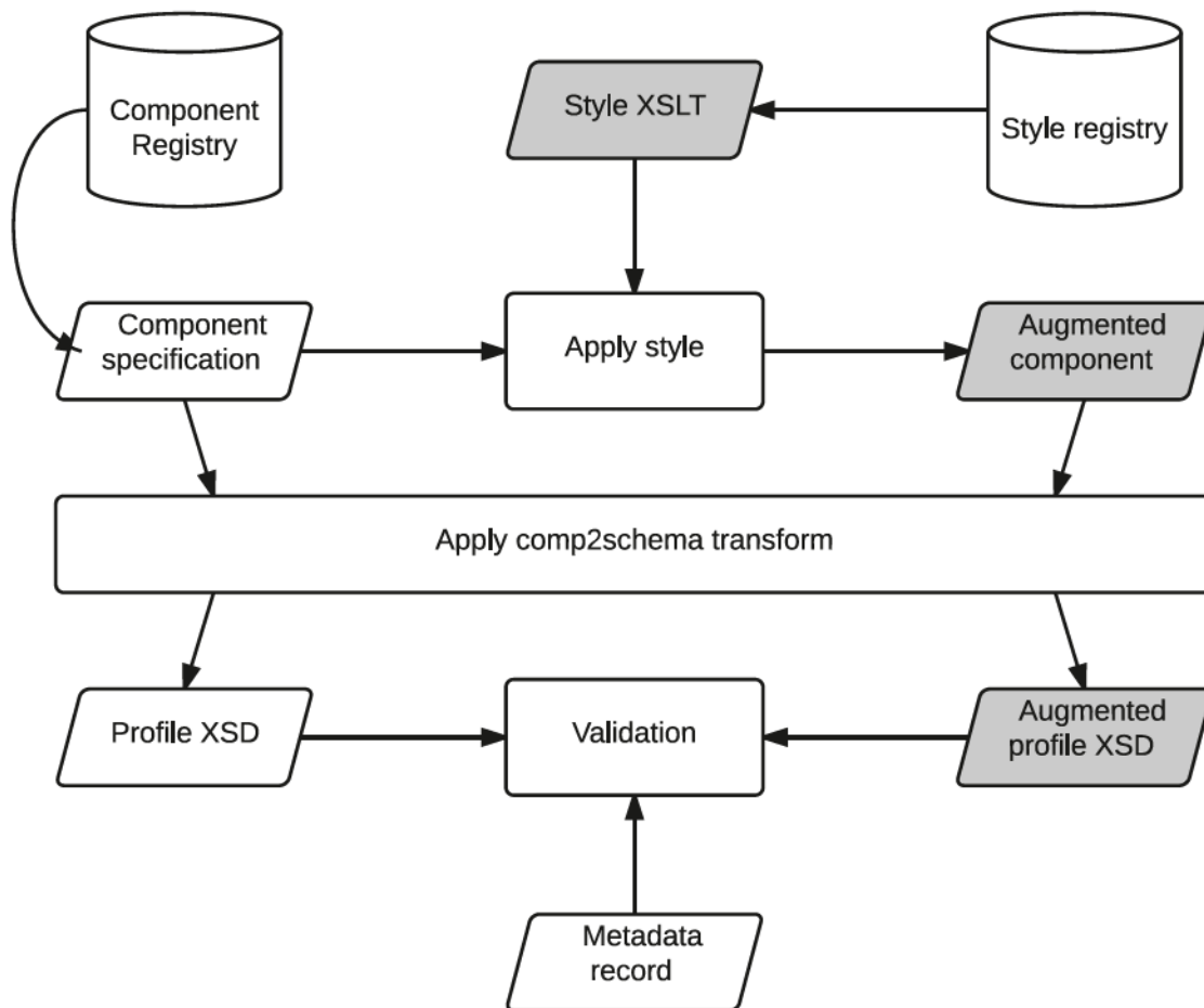
Figure 2: Workflow for visual hints. Shaded components relate to the augmentation of profile schema documents with styling information.
