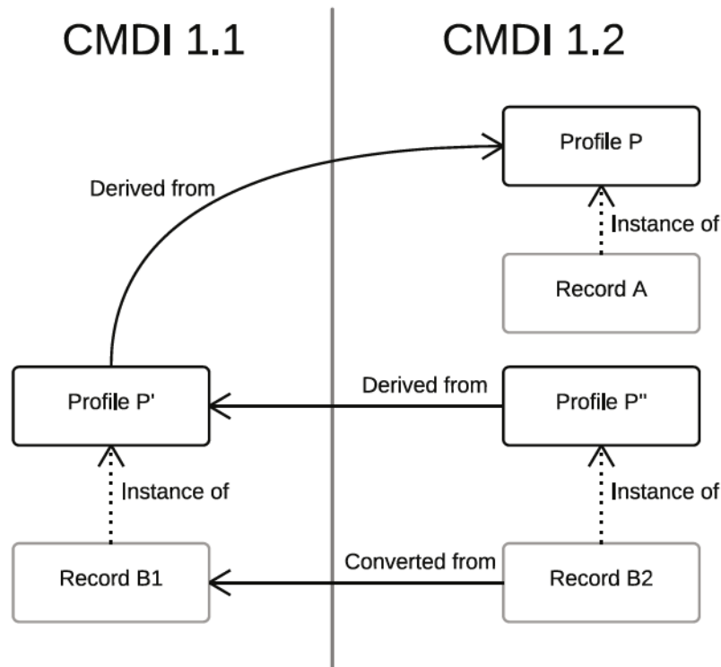
Figure 4: Workflow for a CMDI 1.1 record that is created on basis of a CMDI 1.2 profile and later converted to a CMDI 1.2 instance
