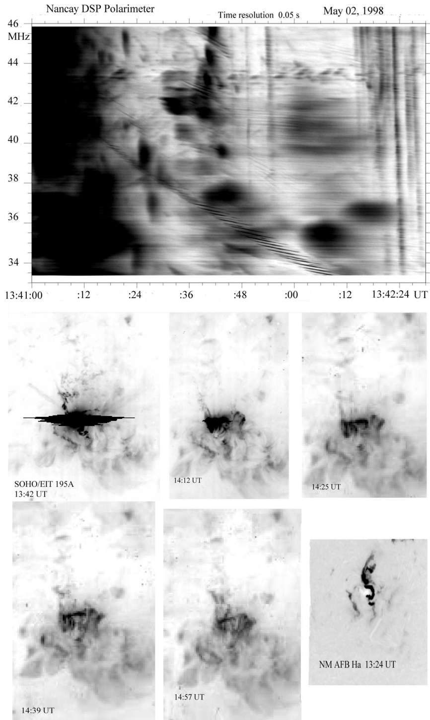
Figure 1: Event 1998 05 02. In the upper panel the dynamic spectra of the Nancay Decameter Spectrometer-Polarimeter are given (summary plot: RH + LH spectral density). In the lower panels the evolution of the flare in the EUV line 195 Å of SOHO/EIT and the H_{\alpha} image of the flare in NOAA AR 7792 are shown.
