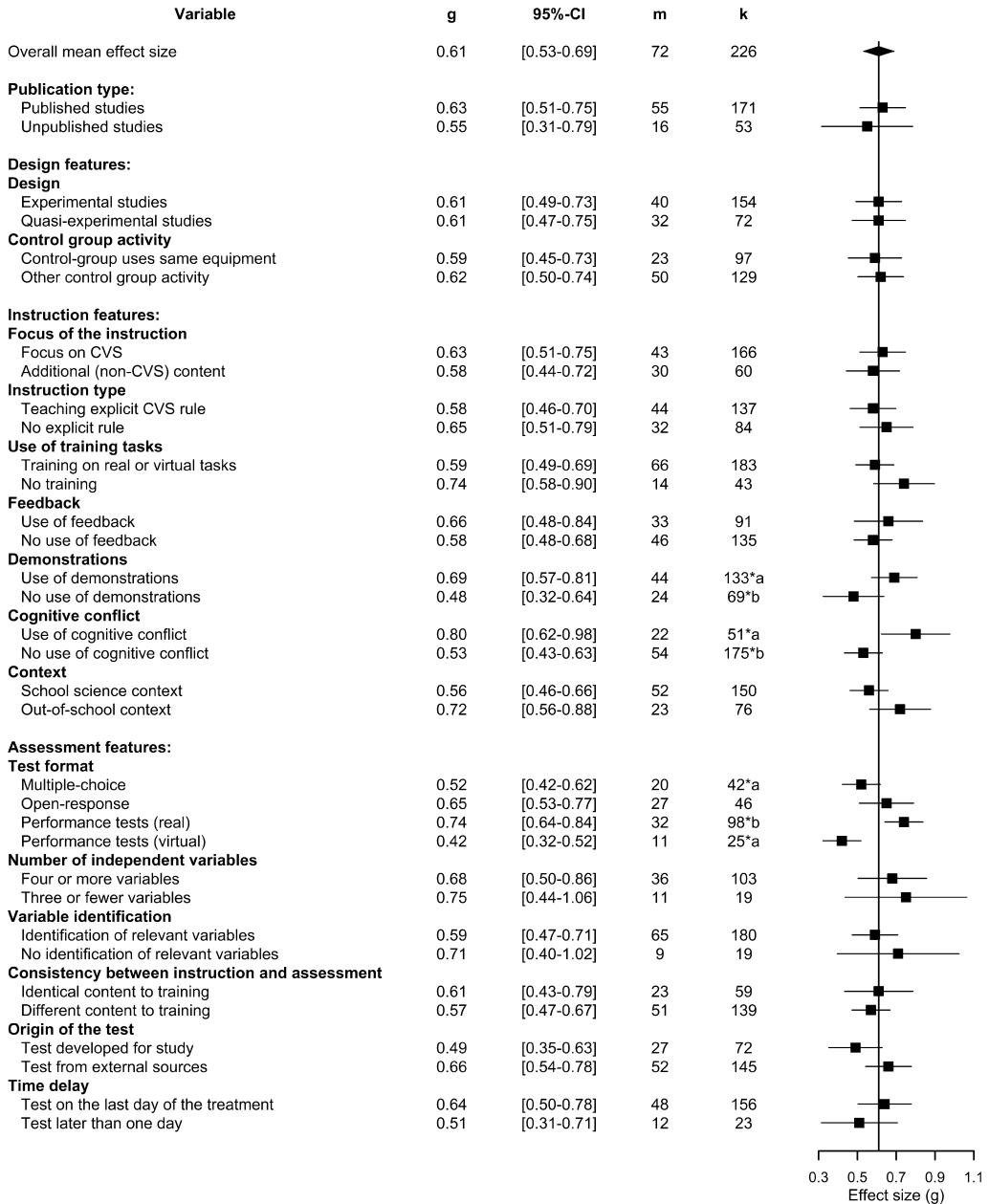
Fig. 4. Forest plot of the moderator effects (g) and 95% confidence intervals (CIs). Note. Items with subscripts a and b mark groups differing from each other at p < 0.05 . The column m refers to the number of studies, and k represents the total number of pairwise comparisons.
