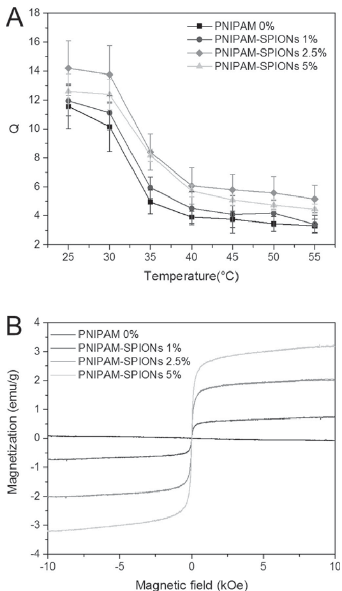
Fig. 3. SPIONs concentration effect on the thermal and magnetic behavior of the hydrogels. Mass swelling ratio (A) from 25 to 55 °C for the hydrogels loaded with different amount of SPIONs (n=3, average \pm SD). Magnetization MH curves of magnetic hydrogels synthesized with different SPIONs concentrations (B).
