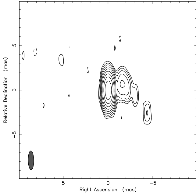
Figure 3. TANAMI image from an 8.4 GHz observation on 2012 September 16. The image peak is 1.29 \text{ Jy/beam} , and the beam (FWHM) is 2.1 \text{ mas} \times 0.6 \text{ mas} at a position angle of 1^\circ . Contour levels are -0.2 (dashed), 0.2, 0.4, 0.8, 1.6, 3.2, 6.4, 12.8, 25.6 and 51.2\% of the peak.
