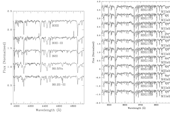
Figure 1. Left. Spectra of the brightest blue members of VdBH 222 and Right. Spectra of red supergiants in and around the open cluster Teutsch 85
