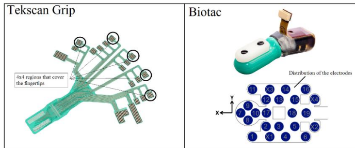
Figure 2: Tekscan Grip sensor used in one hand, where the regions used in the fingertips are marked (left)(source: Tekscan). Biotac sensor and scheme of the distribution of the 19 electrodes inside the sensor (right) (source Syntouch).
