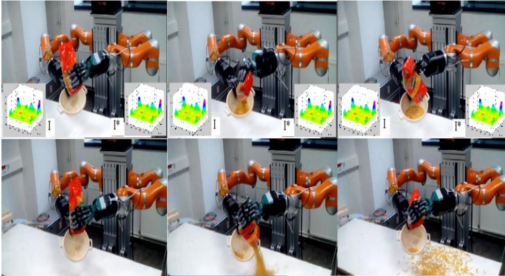
Figure 15: Collaboration experiment using servo-tactile control (up) and without servo-tactile control (down). For the execution with the servo-tactile control, a sample tactile image I is shown (in this case for the index finger). The desired configuration is shown in the image I^* .
