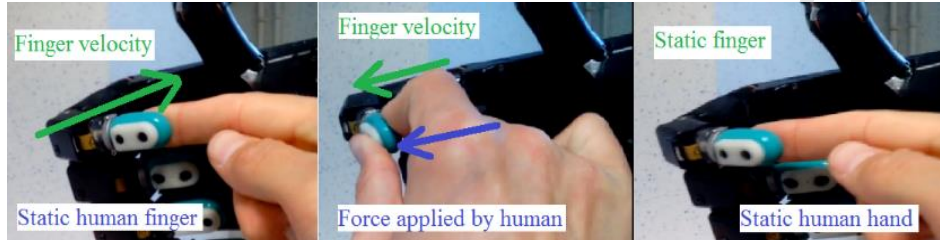
Figure 7: Experiment with the servo-tactile control, different steps. Controlling the magnitude of the force in the contact.
