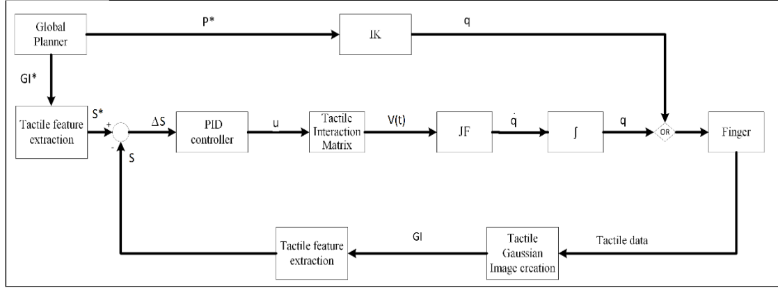
Figure 6: Control diagram of the servo-tactile architecture executed on each finger f_i .
