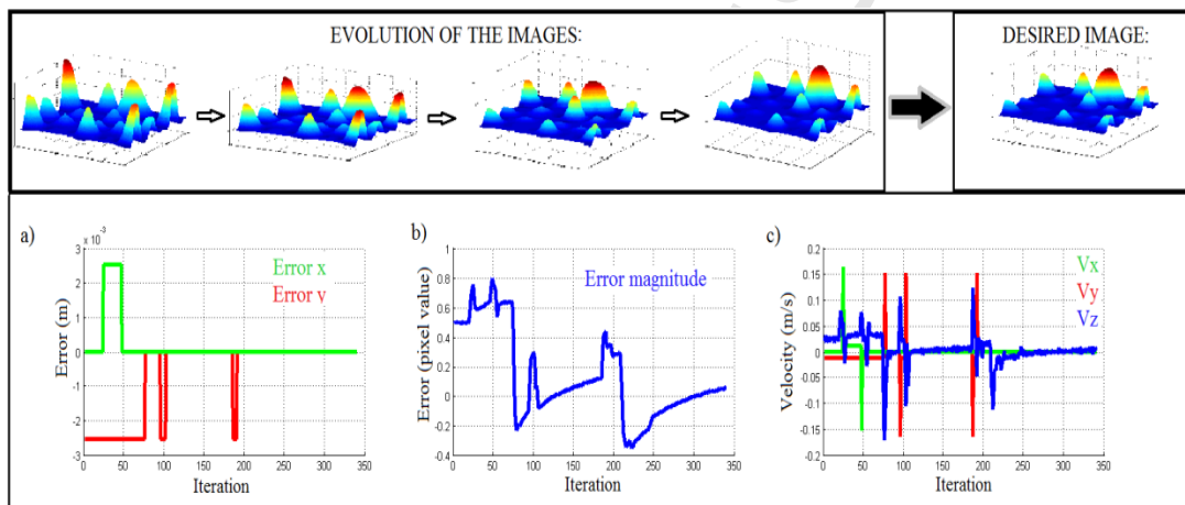
Figure 8: Evolution of error (a, b), velocities (c) and sample and desired tactile images (above).
