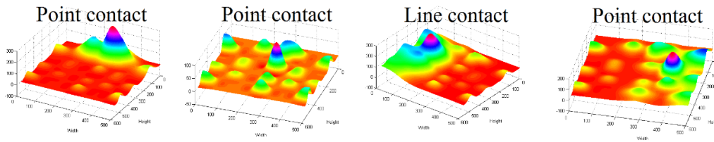
Figure 4: Different tactile images obtained with the mixture of Gaussians method for different contact configurations. From left to right: point contact on the finger end, central point contact, lineal contact on left side, and point contact on the right side.
