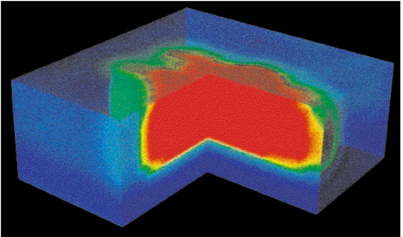
During the IronEx II experiment in the eastern equatorial Pacific, investigators fertilized an area of 64 km 2 with iron. Phytoplankton photochemical quantum efficiency (the fraction of absorbed photons used in photosynthesis) increased in the area enriched with iron from less than 0.3 (blue) to greater than 0.55 (red) in surface waters down to 30 meters depth. Reproduced from (8).
