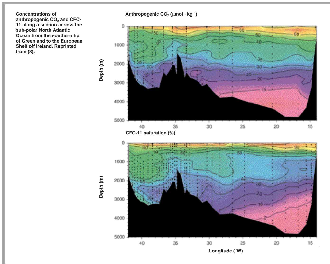
Figure 5. Anthropogenic Tracers in the North Atlantic.
