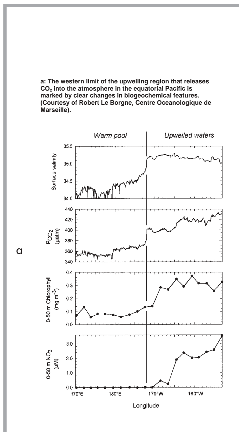
Figure 11. Climate, Physics and the Air-Sea Flux of CO 2 in the Equatorial Pacific.
