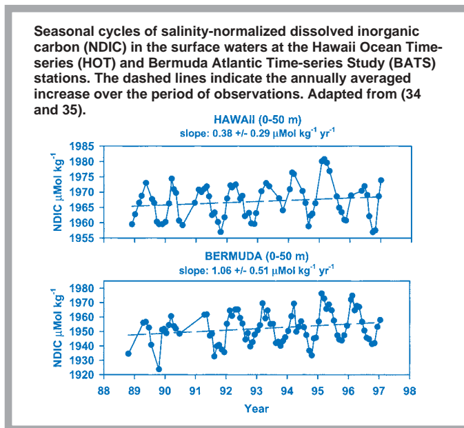
Figure 17. Measuring the Anthropogenic Impact on Ocean DIC Concentrations.
