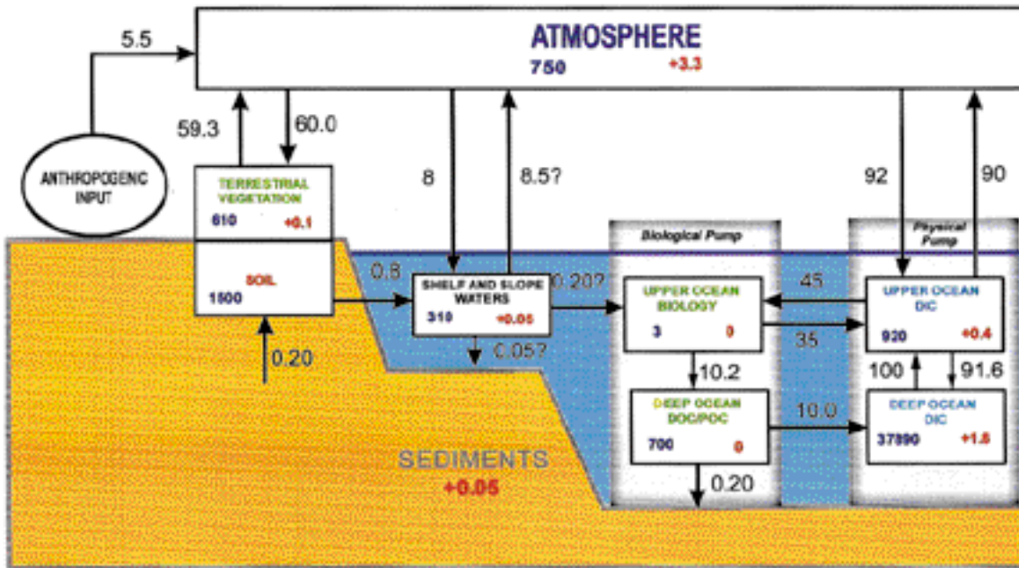
Average annual fluxes between global carbon pools are given in petagrams of carbon per year ( \text{Pg C yr}^{-1} ). Figures in blue in each box denote the global inventory in Pg C, while figures in red show the average annual increases in the inventory associated with anthropogenic input. The fluxes associated with the shelf and slope waters are still uncertain. Figure based on the 1995 Intergovernmental Panel on Climate Change (IPCC) analysis with additions from JGOFIS results.
