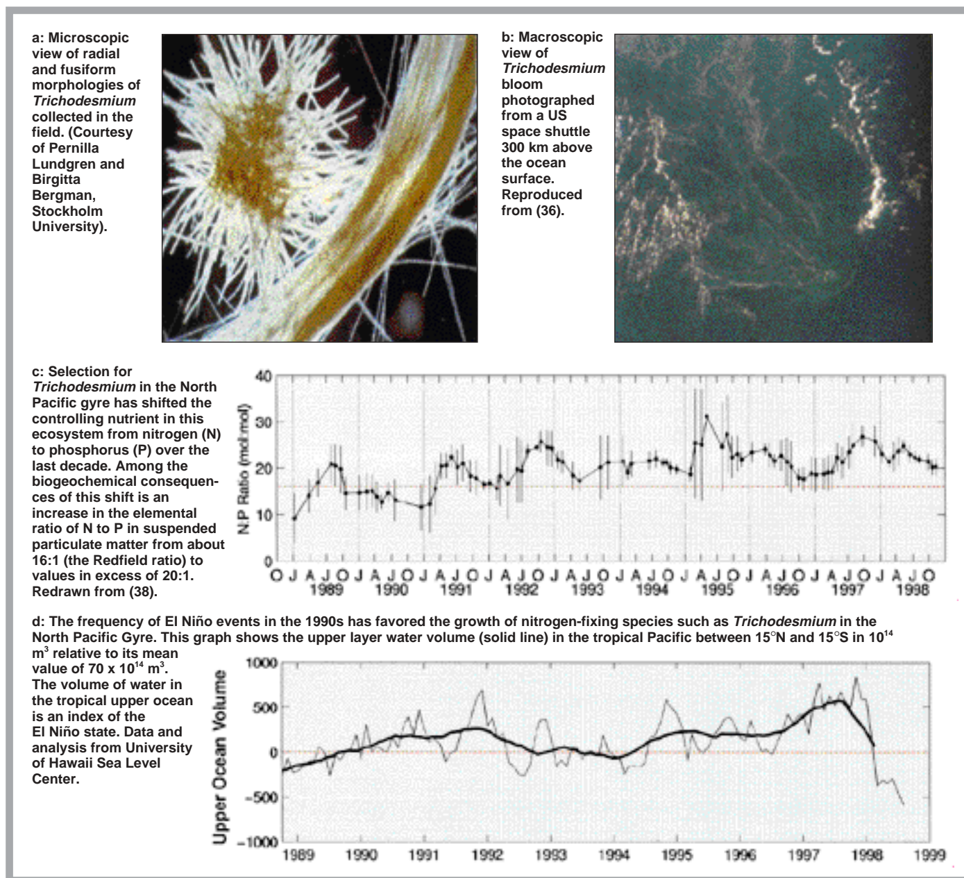
Figure 18. Climate, Nitrogen Fixation and Ecosystem Change.
