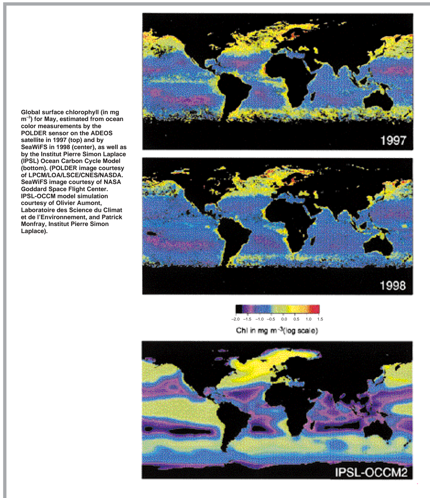
Figure 22. Third Generation of Ocean Carbon Cycle Models.
