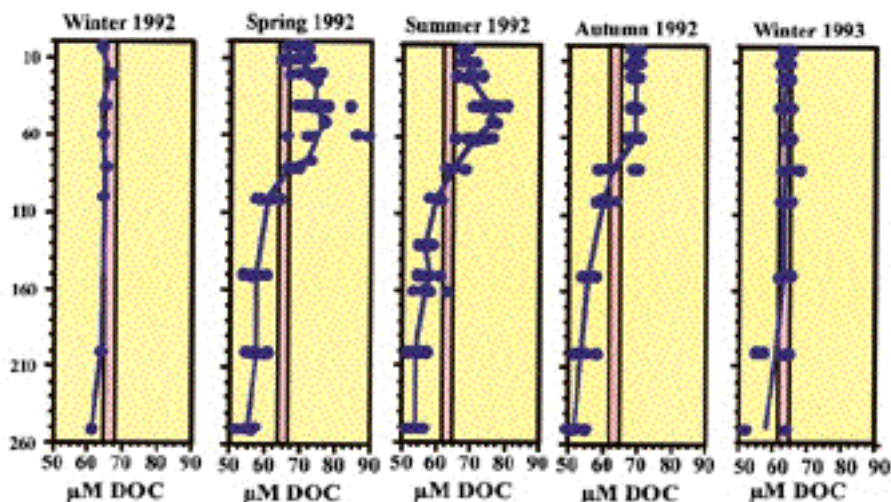
b: Vertical profiles of DOC measurements at the BATS site (31°50'N, 64°10'W) over one year (1992). The red bars indicate the average range of DOC values (micromolar) during deep mixing in the winter. Redrawn from (19).
