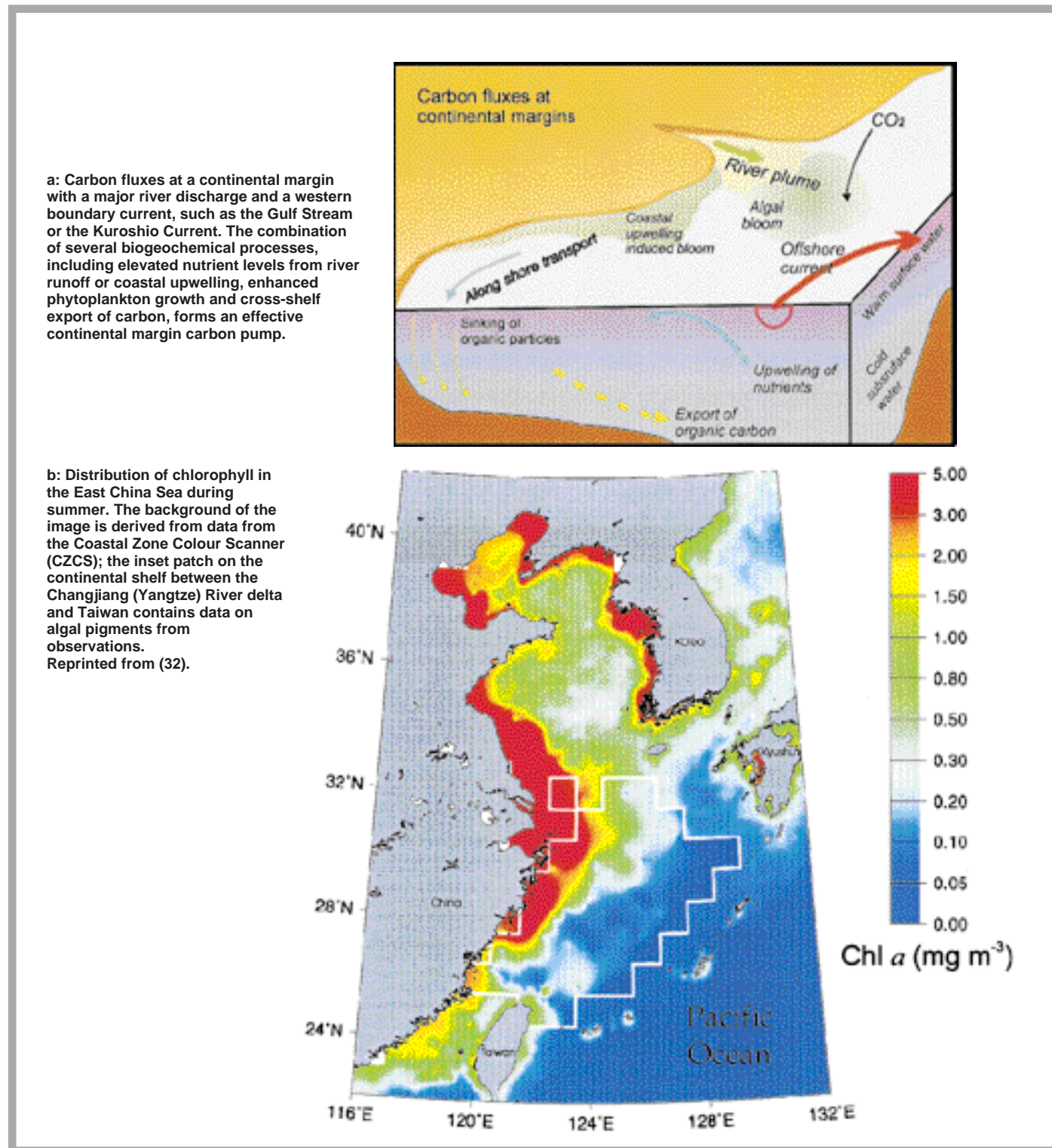
Figure 16. Carbon Fluxes in the Continental Margins.
