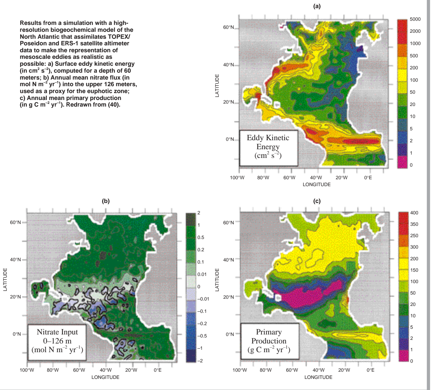
Figure 21. Three-dimensional Modelling on the Regional Scale.
