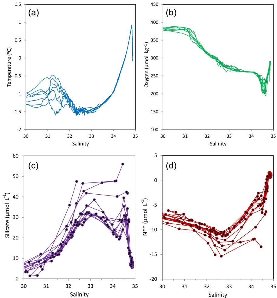
Figure 8. Temperature (a), oxygen (b), silicate (c) and N^{**} (d) versus salinity for the stations at sections D and E. The panels (a) and (b) are from the CTD output, while (c) and (d) are from water samples analysed.
