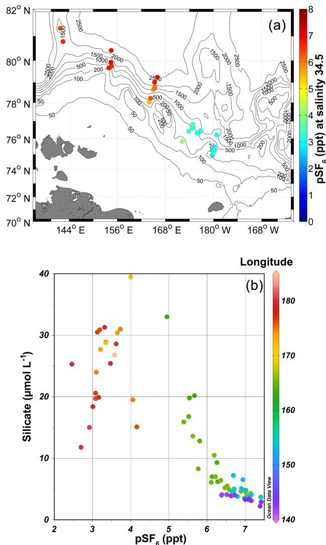
Figure 9. SF 6 partial pressure (ppt) interpolated to the salinity 34.5 (a) and silicate versus pSF 6 in the salinity range 34.3 to 34.7 colour coded by longitude (b).
