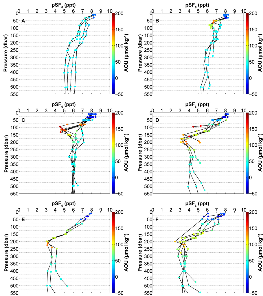
Figure 5. pSF 6 (ppt per volume) profiles from surface to 550 m depth, coloured by AOU (μmol kg -1 ) of the stations in sections A to F.
