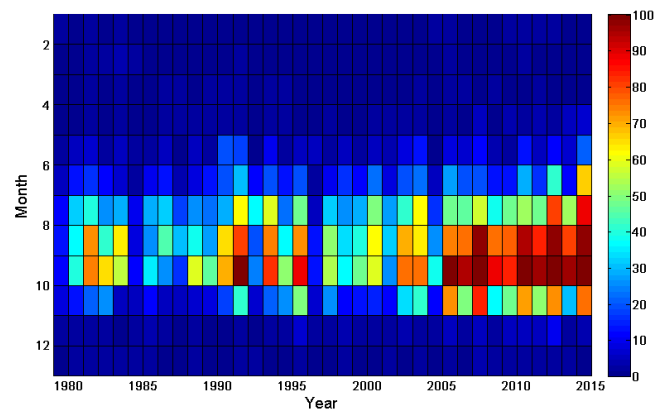
Figure 12. Percentage of ice-free area in the region: latitude 76 to 80° N, longitude 140 to 150° E (framed yellow in Fig. 1b), for each month from 1980 to 2014, evaluated from the passive microwave data of NSIDC (Cavalieri et al., 1996).
