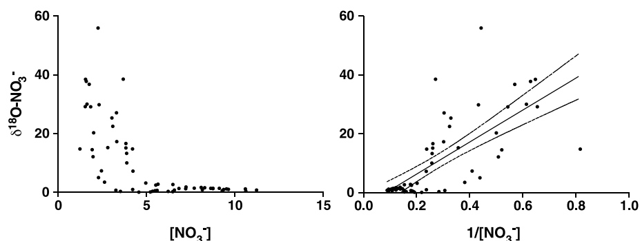
Figure 6. The \delta^{18}\text{O} of the nitrate against (left) the nitrate concentration and against (right) the inverse nitrate concentration with the linear regression (black line) and its 95% confidence interval (dashed lines).
